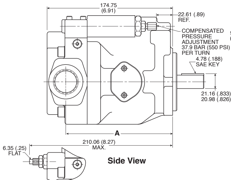
ADJ. MAX. VOLUME STOP (1.6 CC/REV/TURN) "OPTION 2"
